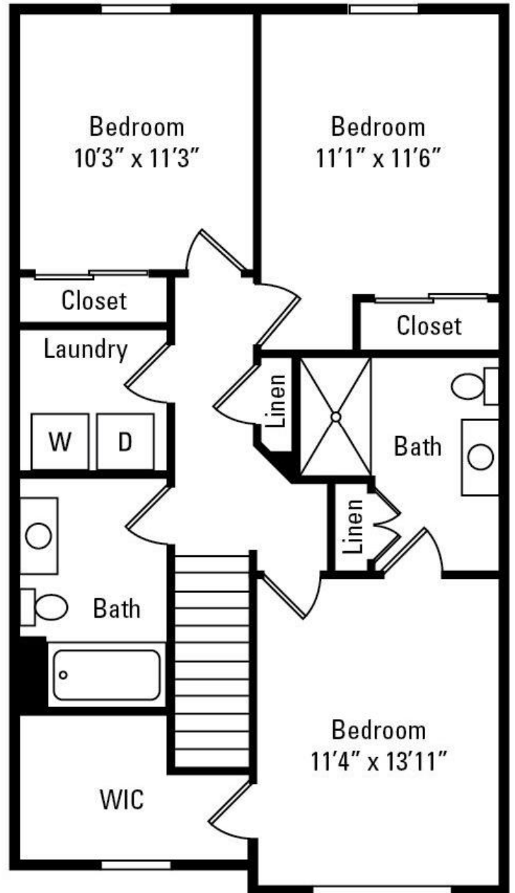
2nd Floor
